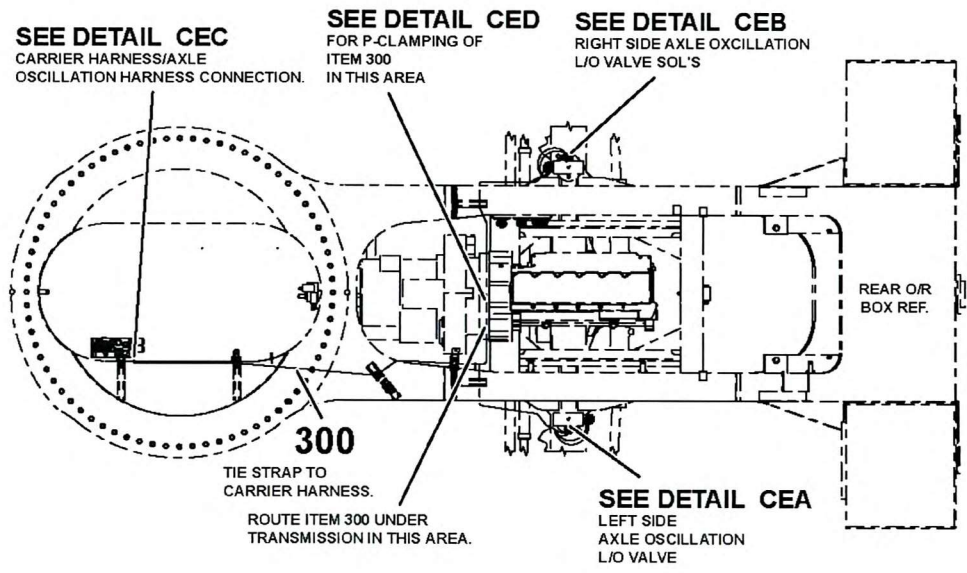
ELEC CE COMPONENTS TOP VIEW OF CARRIER
